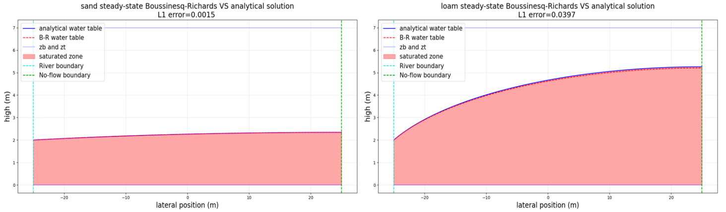
Figure 2: Comparison between the Boussinesq-Richards numerical solution and the analytical solution.
