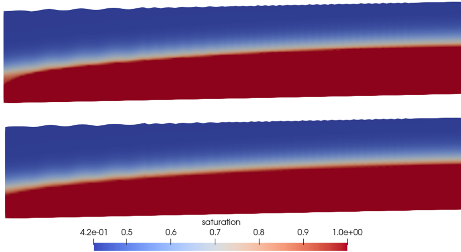
Figure 15: Steady-state saturation results. Top: Boussinesq-Richards; Bottom: Richards.
