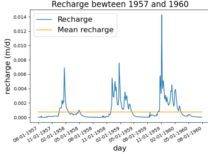
Figure 14: Recharge from 1957 to 1960
